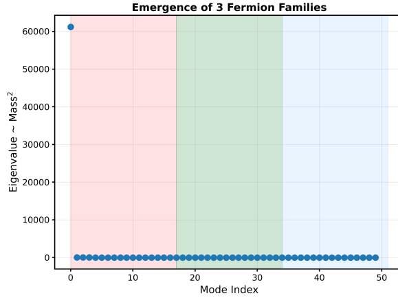
Figure 1: Emergence of 3 Fermion Families. The spectrum shows 3 distinct blocks.
