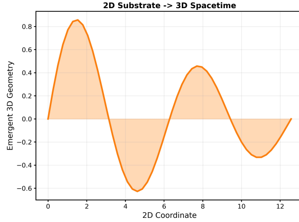
Figure 3: 2D Substrate \rightarrow 3D Spacetime. The excitation is the geometry.
