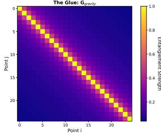
Figure 4: The Glue: G_{gravity} . Map of entanglement in the 2D substrate.
